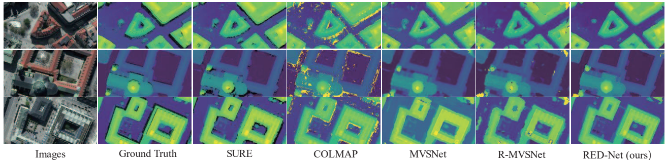
Figure 6: The inferred depth maps of three sub-units on München aerial image set. The deep learning based methods are trained on the WHU-3 training set.
